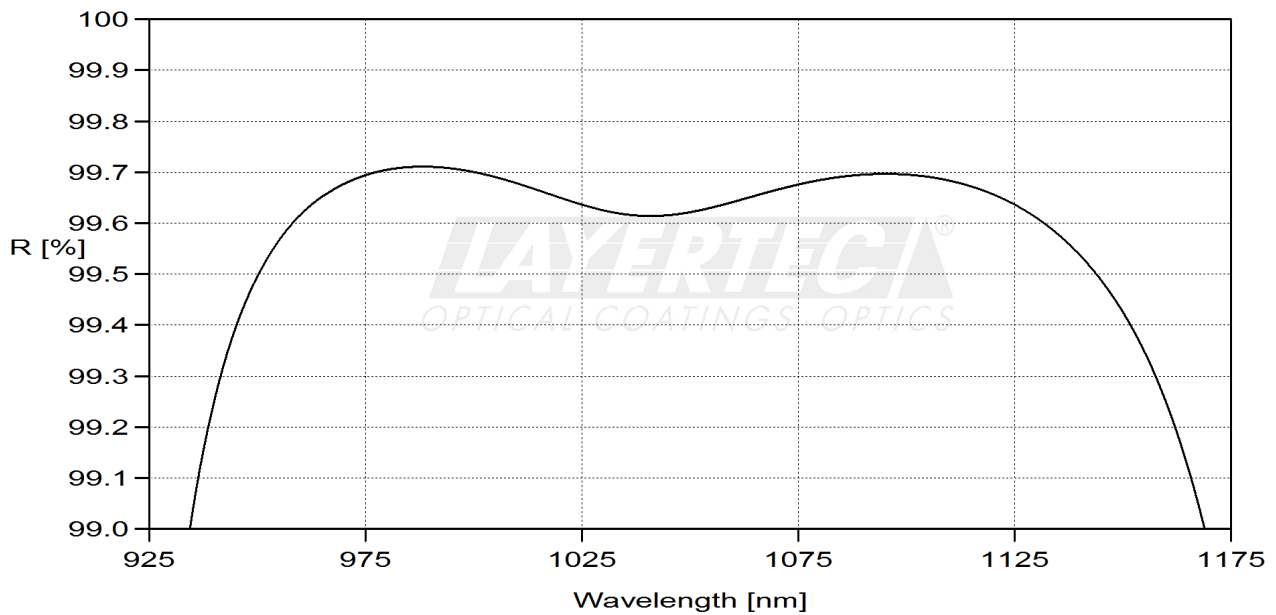
fig. 2 reflection PR-region 0° (zoomed from fig. 1)
