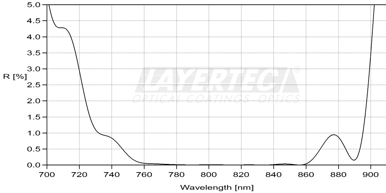
fig. 2 reflection R-region 0°
