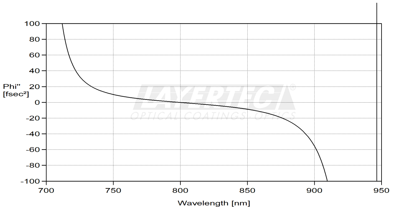
fig. 2 calculated GDD(R,0°)
