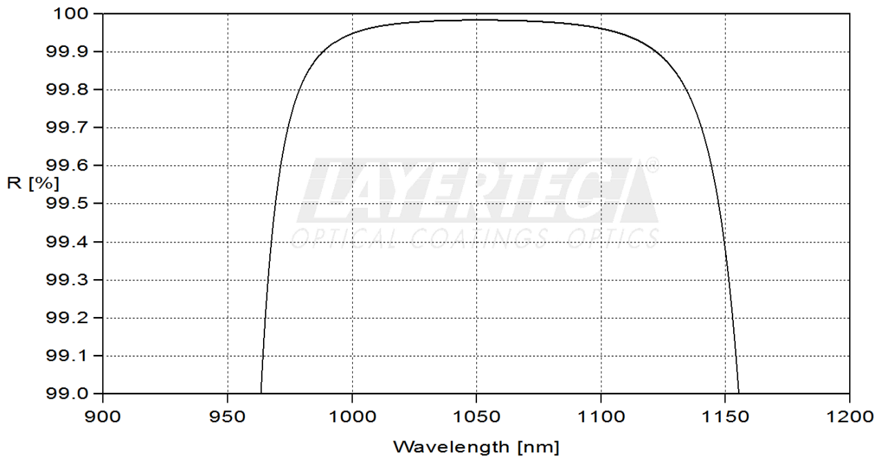
fig. 1 calculated reflection 0°
