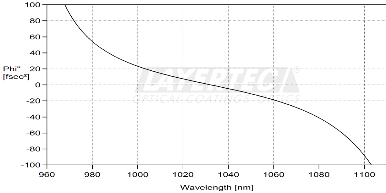
fig. 1 calculated GDD(R,0°)
