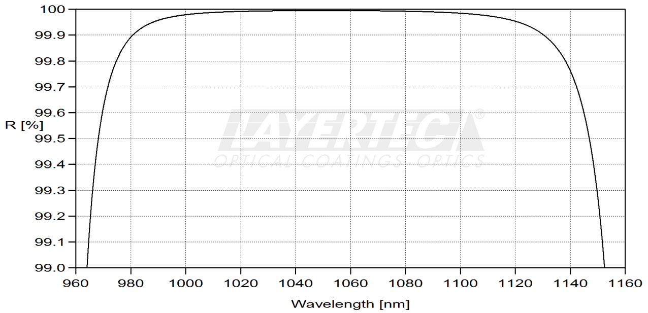
fig. 2 reflection HR-region 0°
