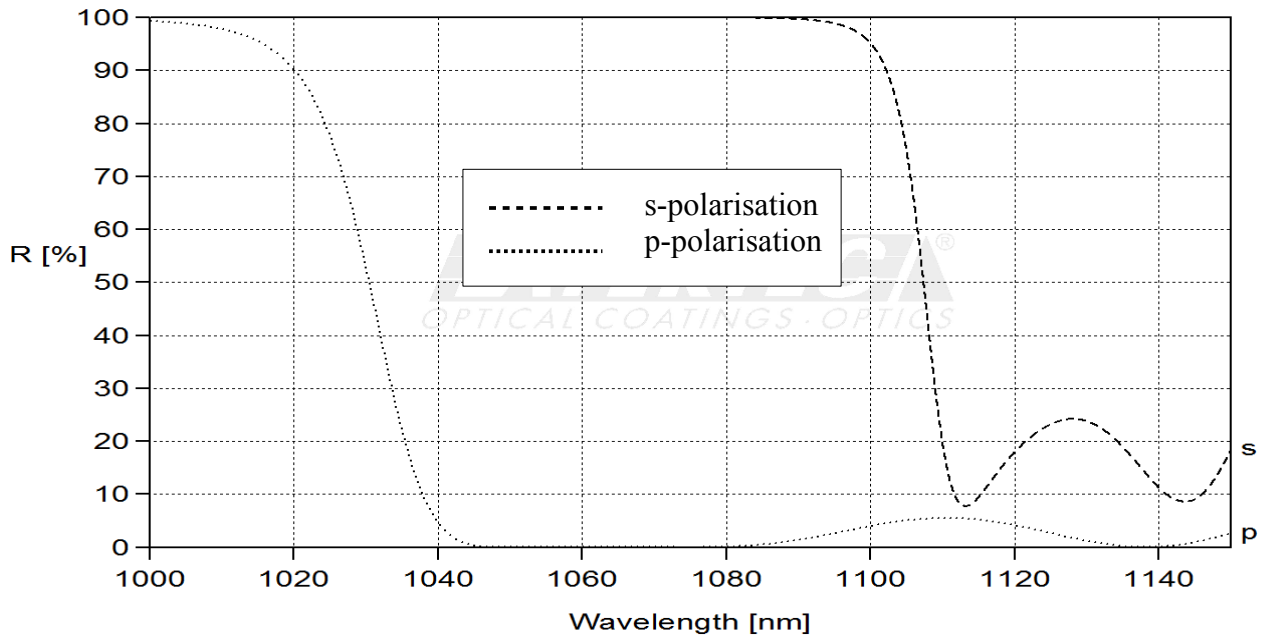
fig. 1 reflection for p- and s-polarisation for AOI=57°
