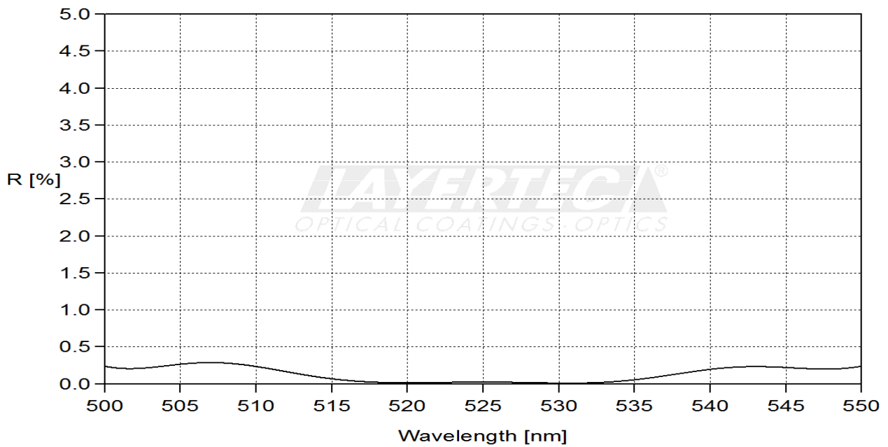
fig. 2 reflection HT-region 0°
