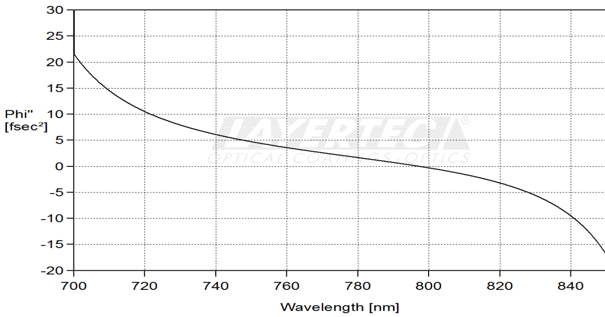
fig. 3 calculated GDD(R,0°)
