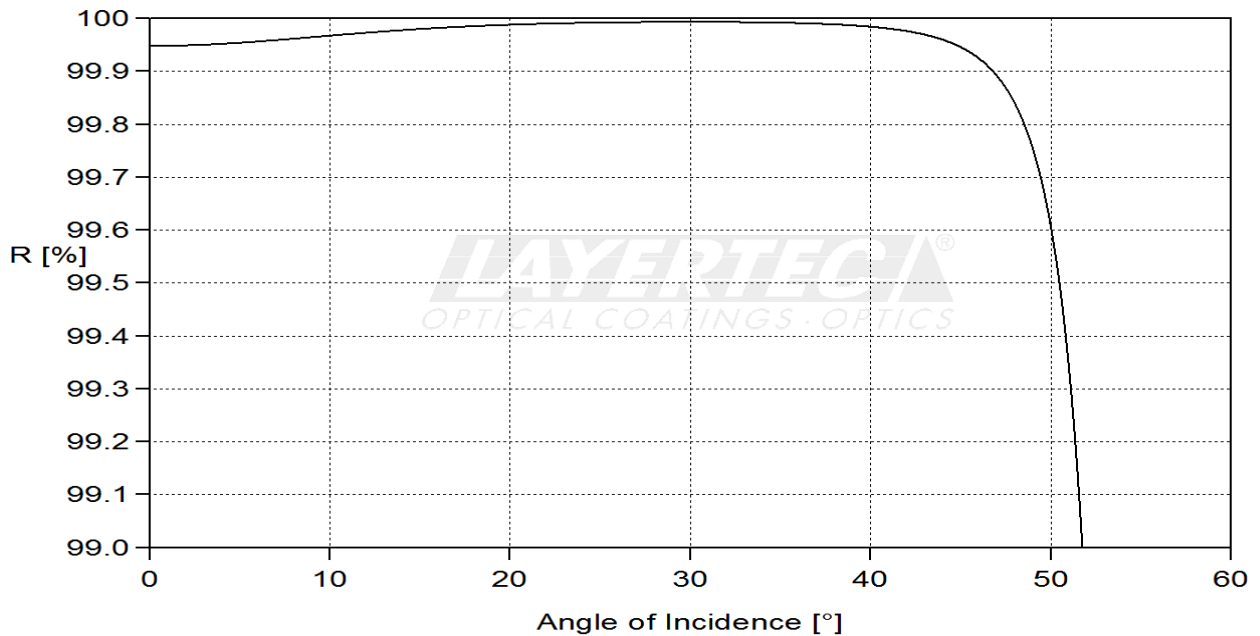
fig. 1 reflection versus AOI for \lambda = 1064\text{nm} (unpolarized)
