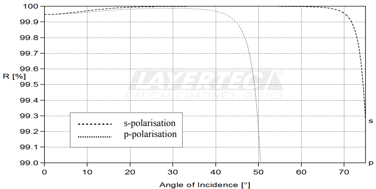
fig. 2 reflection versus AOI for \lambda = 1064\text{nm}
