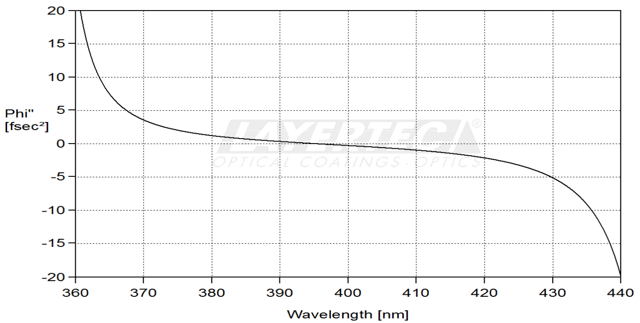
fig. 2 calculated GDD(R,0°)
