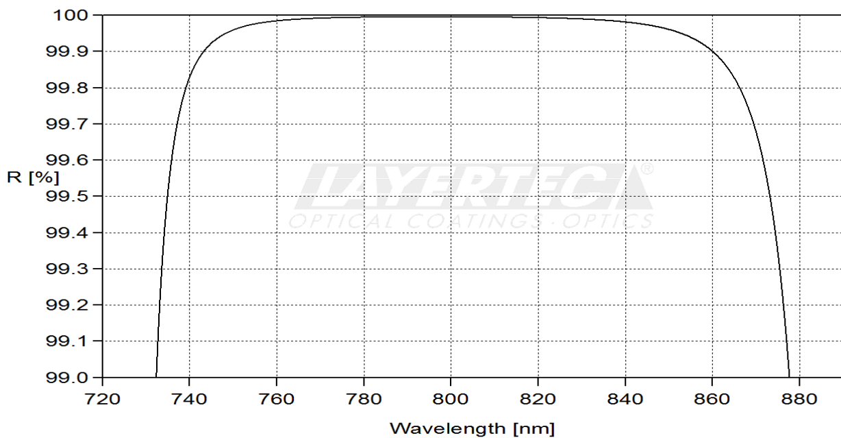
fig. 2 reflection HR-region 0°
