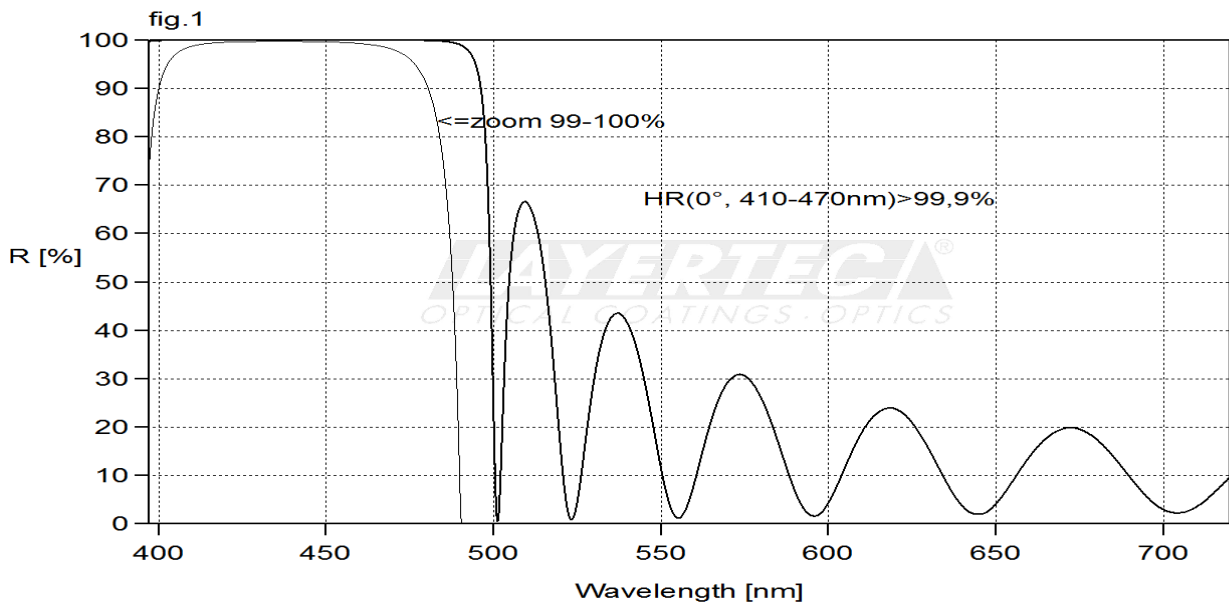
fig. 1 calculated reflection 0°
