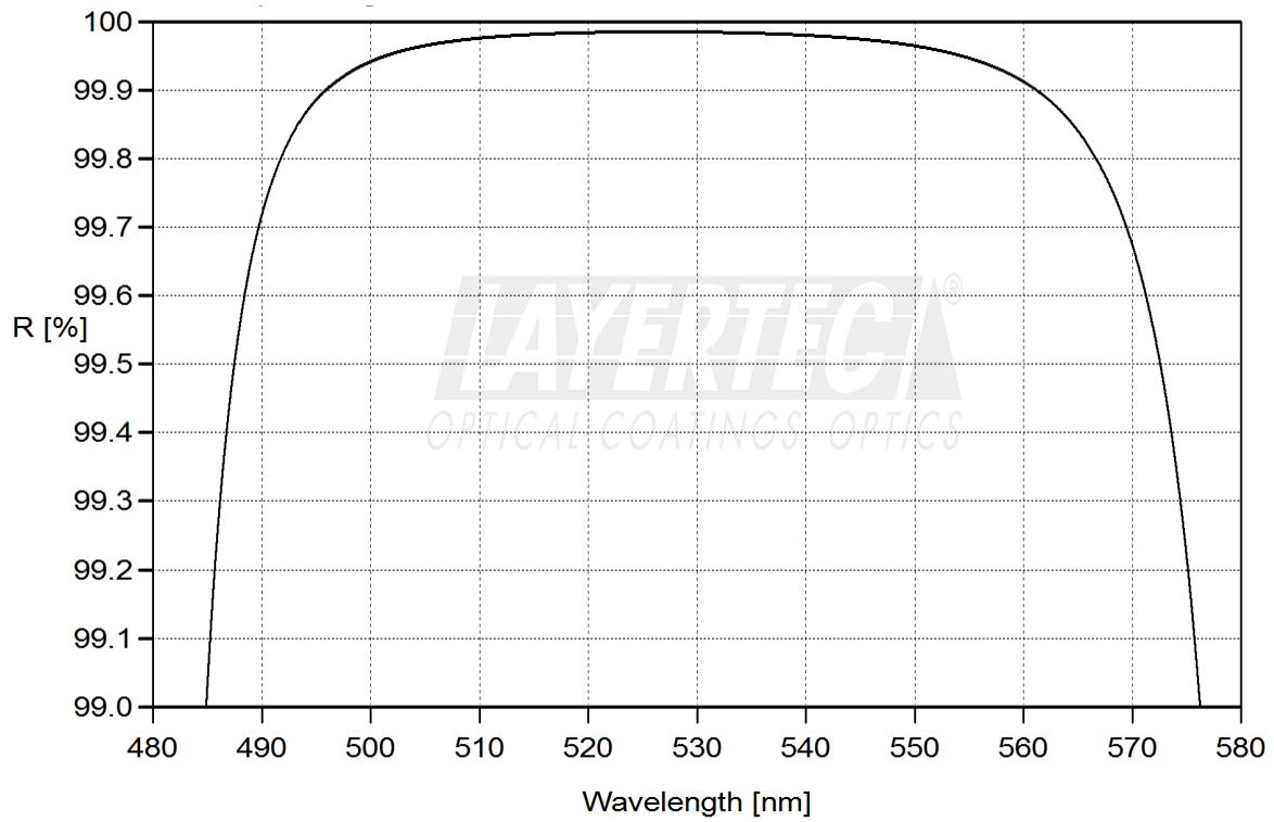
fig. 1.1: HR (45°, 532nm) > 99.9%
