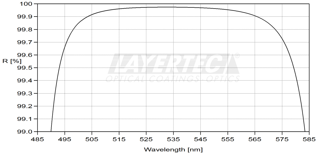
fig. 1 reflection HR-region 0°
