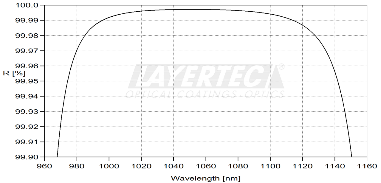
fig. 1 reflection HR-region 0°
