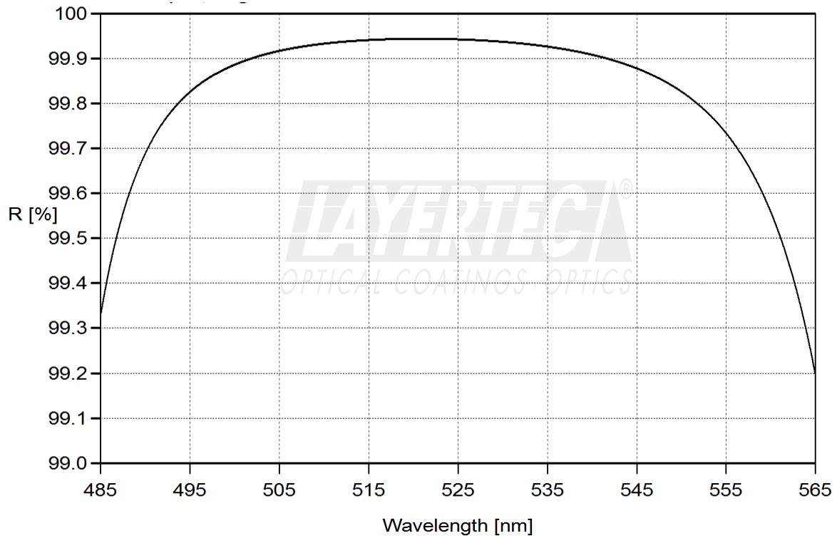
fig. 1.1: HRu (45°, 514 - 532nm) > 99.8%
