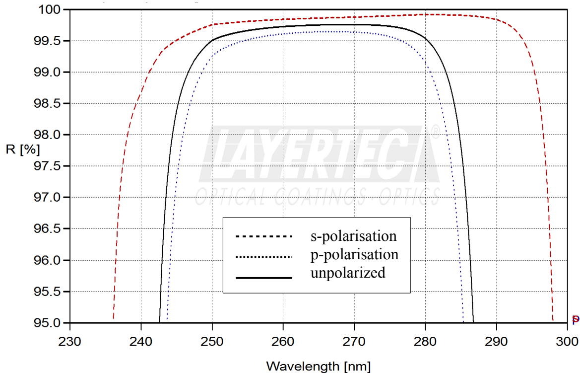
fig. 1.1: HRr (45°, 266nm) > 99.5%
