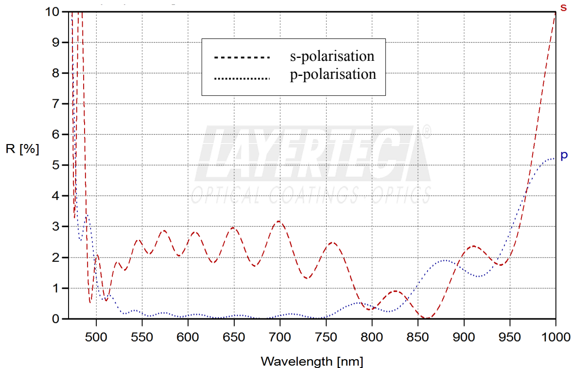
fig. 1.2: Rs,p (45°, 500 - 930nm) < 5.0% + Rs,p (45°, 800nm) < 2% +
