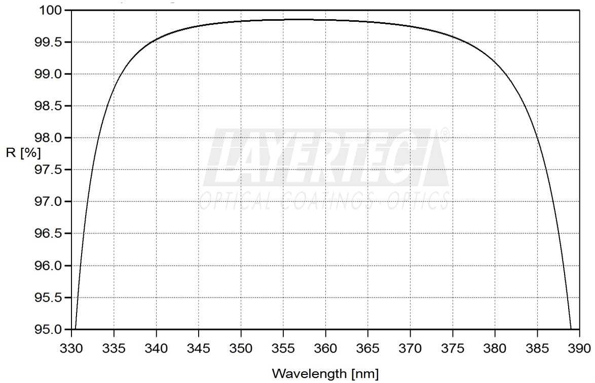
fig. 1.1: HRr (45°, 355nm) > 99.5%
