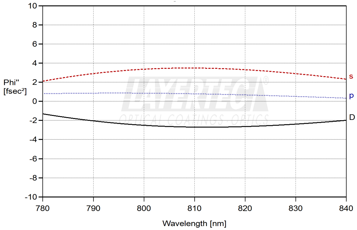
fig. 1.: GDD – T at 810nm (for s-, p- and random)
