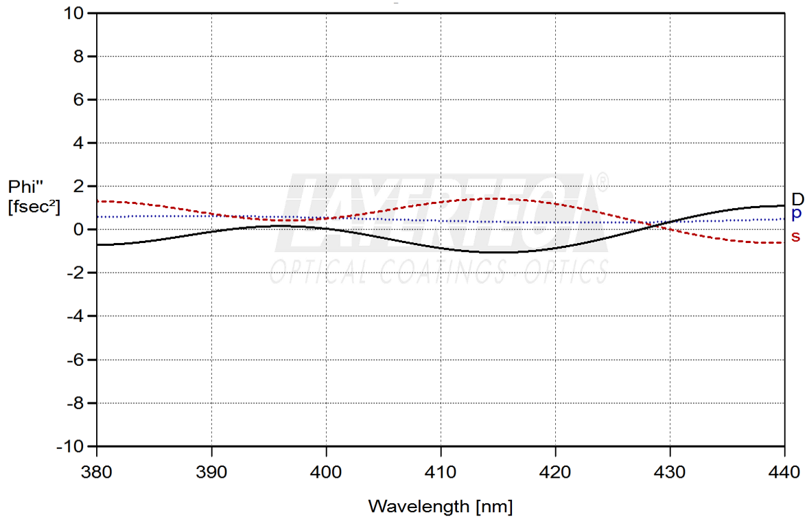
fig. 1.2: GDD – T at 405nm (for s-, p- and random)
