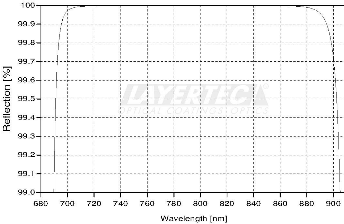
fig. 1: calculated reflectivity
