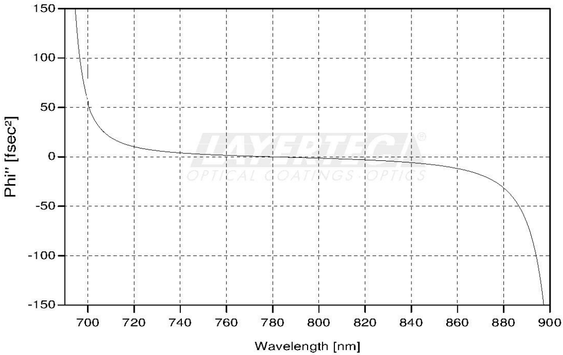
fig. 2: calculated GDD, reflected beam
