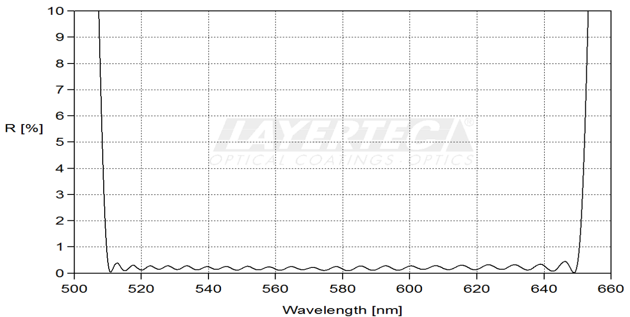
fig. 2 reflection R-region 10° (unpolarized)
