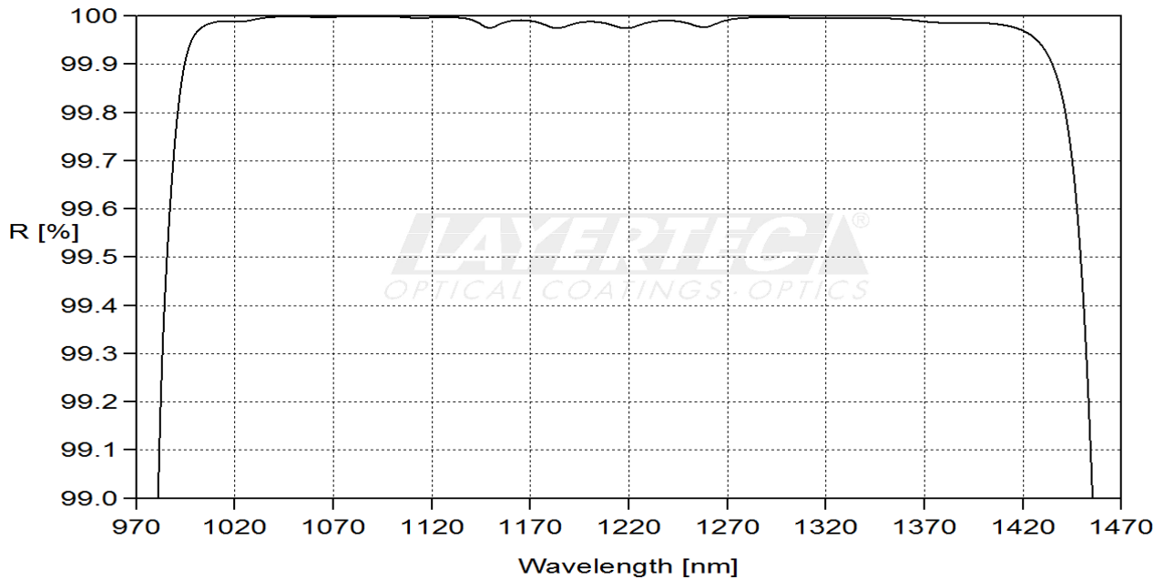
fig. 1 reflection HR-region 10° (unpolarized)
