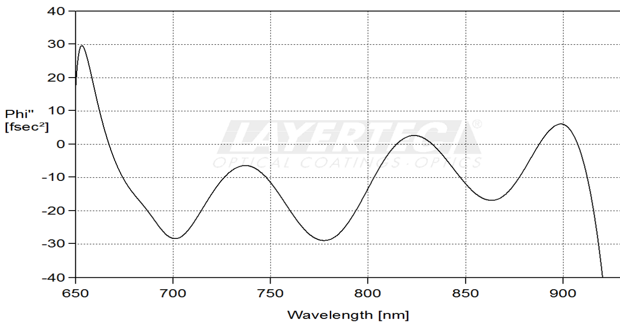
fig. 2 calculated GDD(R,0°)
