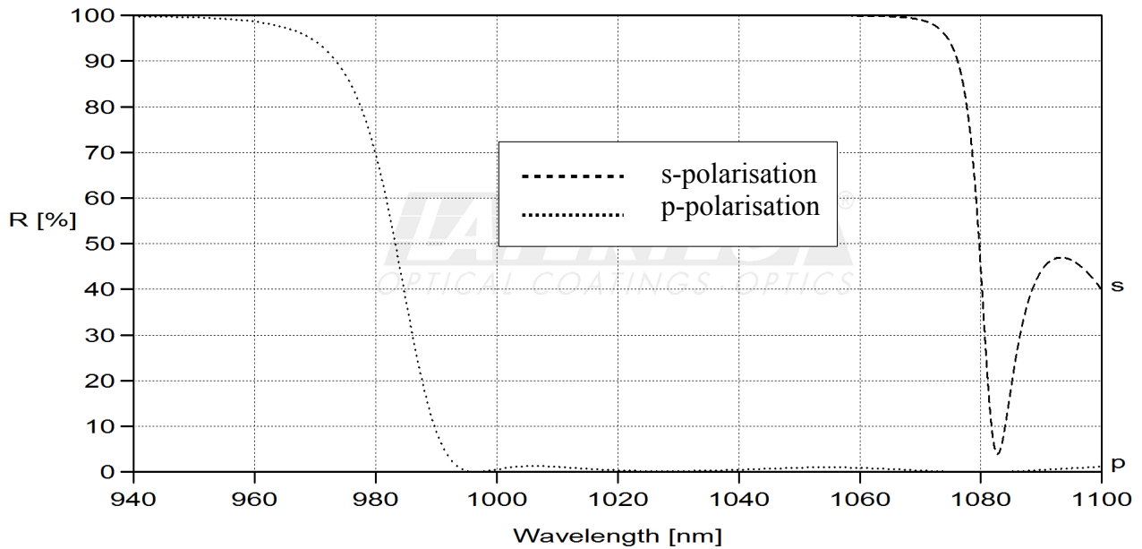
fig. 1 reflection for p- and s-polarisation for AOI=66°
