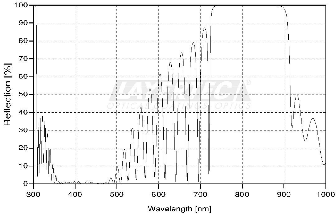
fig. 2: calculated reflectivity @ HR region
