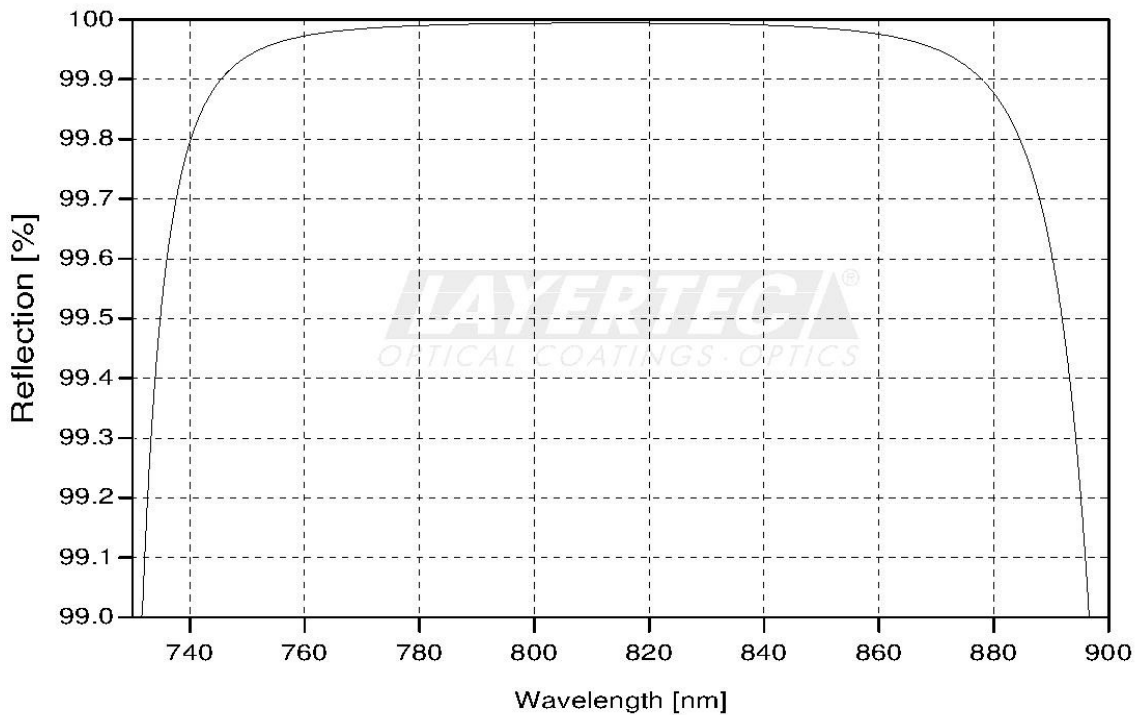
fig. 2: calculated reflectivity @ HR region
