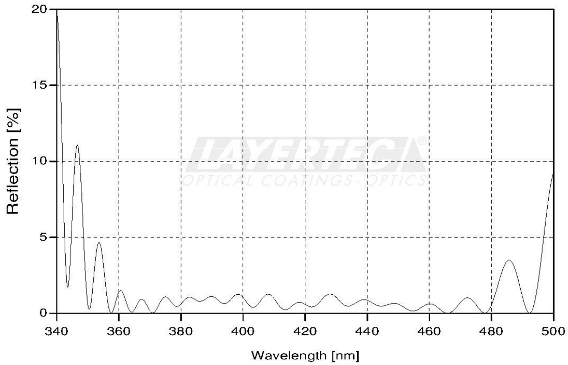
fig. 3: calculated reflectivity @ HT region
