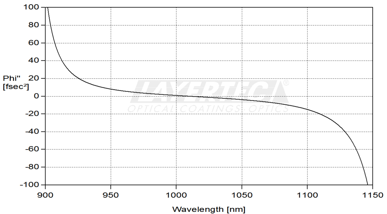
fig. 2 calculated GDD(R, 0°)
