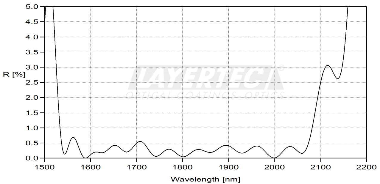
fig. 2 reflection R-region 0°
