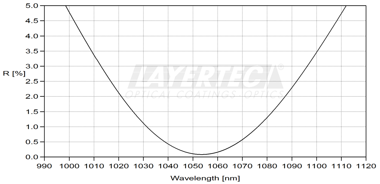
fig. 3 reflection R-region 0°
