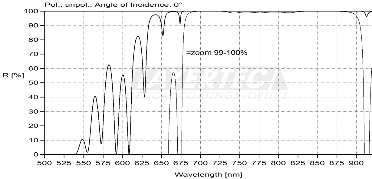
fig. 2 calculated GDD-Rp, 0°
