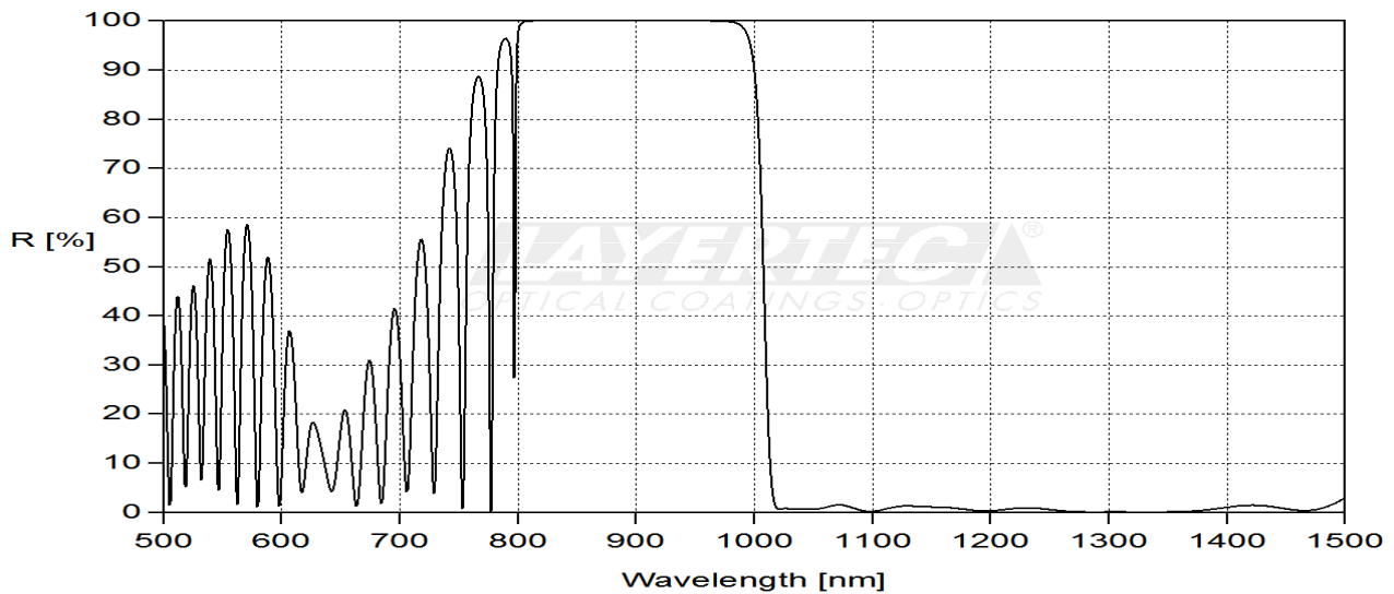
fig. 2 detail cut on/off-region reflection, 0°, please note the production tolerance
