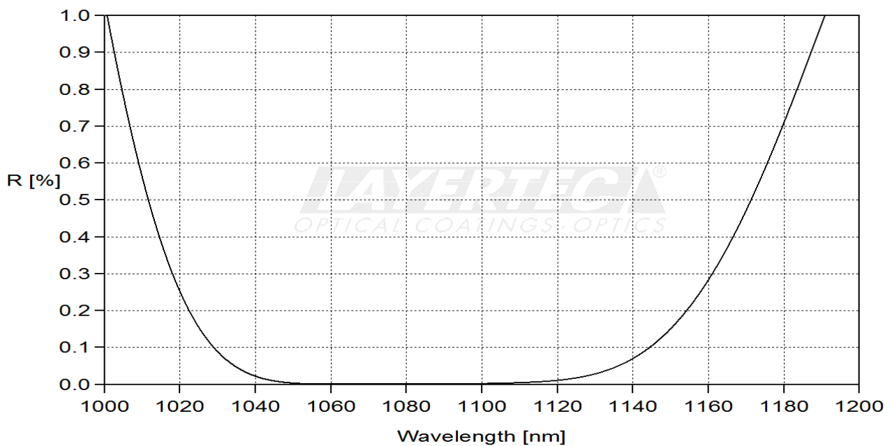
fig. 2 reflection R-region 0°
