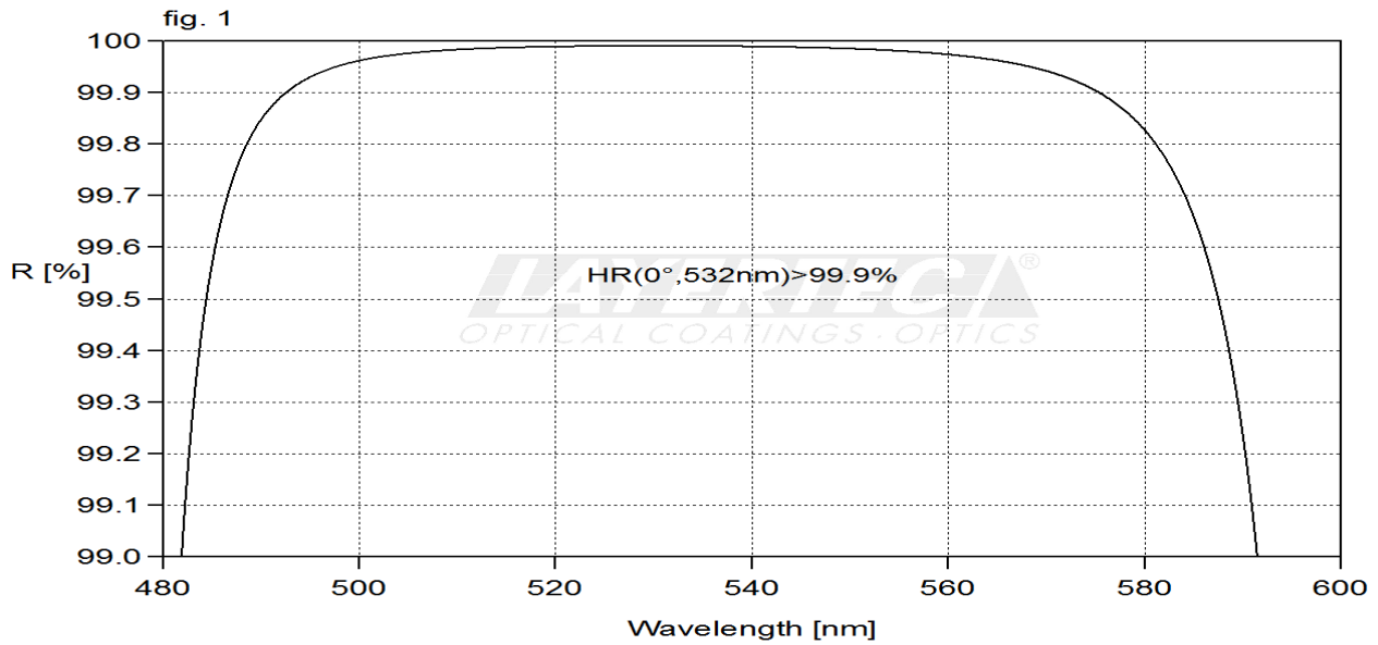
fig. 1 reflection, 0° unpol.
