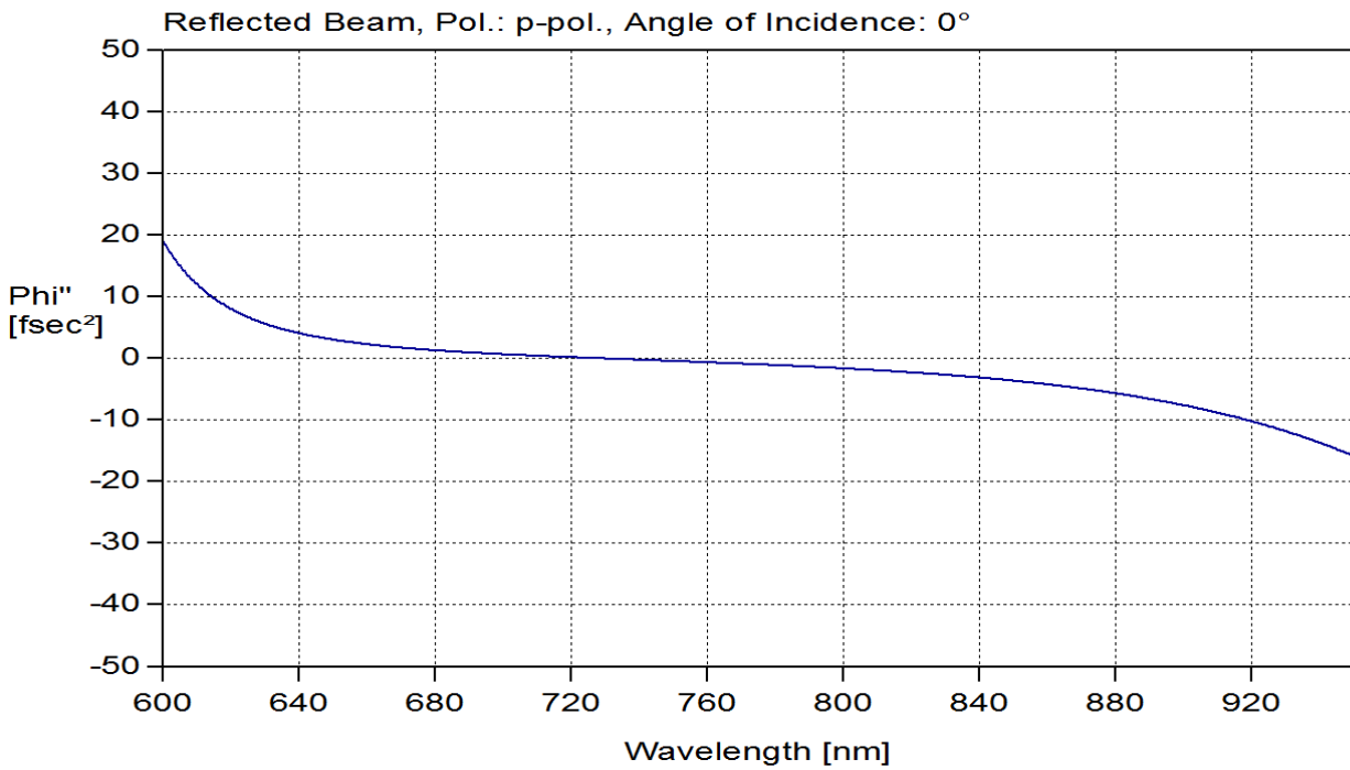
fig. 2 calculated GDD-R
