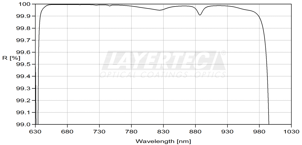
fig. 1 reflection HR-region
