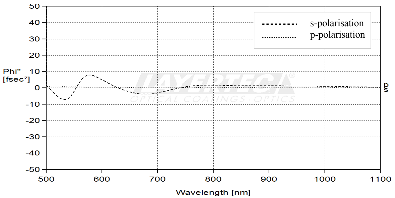
fig. 2 calculated GDD(T,45°)
