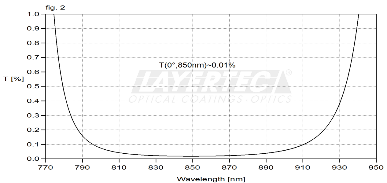
fig. 2 transmission, 0°
