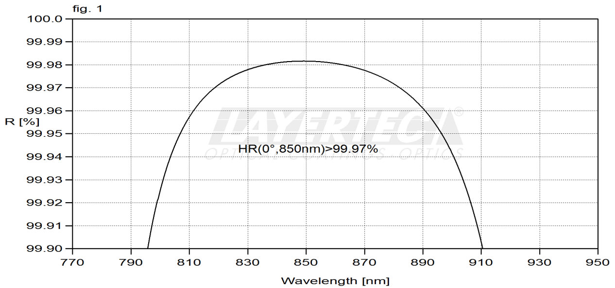
fig. 1 reflectance, 0°
