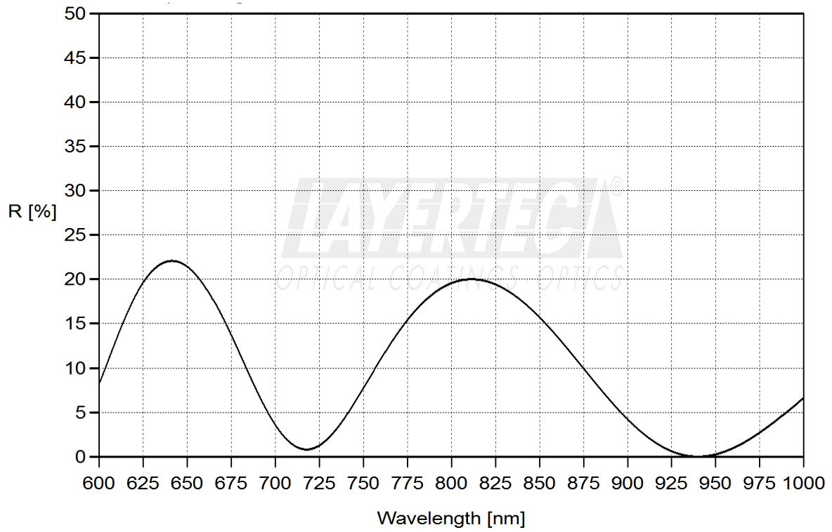
fig. 1.3: theoretical reflexion of coating 114118 in the IR range.
