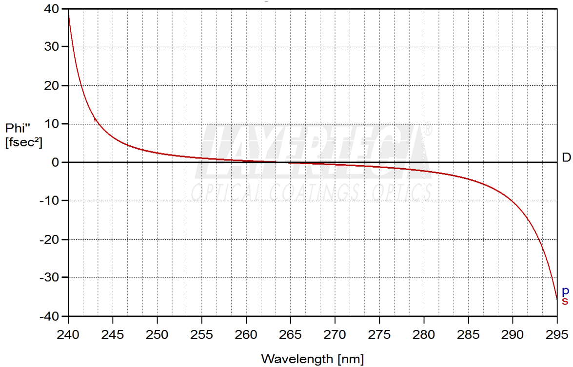
fig. 1.1: GDD in HR region at 266\text{nm} < 20\text{fsec}^2
