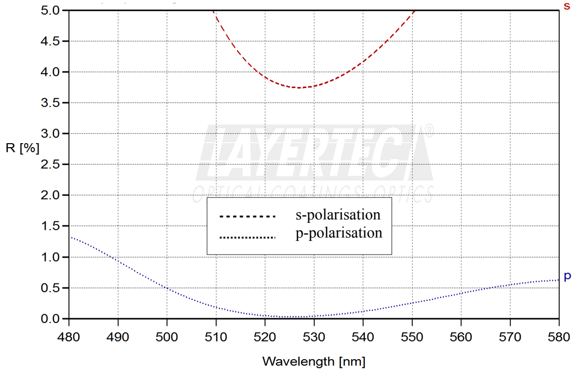
fig. 1.2: Rp (45°, 532nm) < 2.0% + Rs(45°, 532nm) < 10.0%
