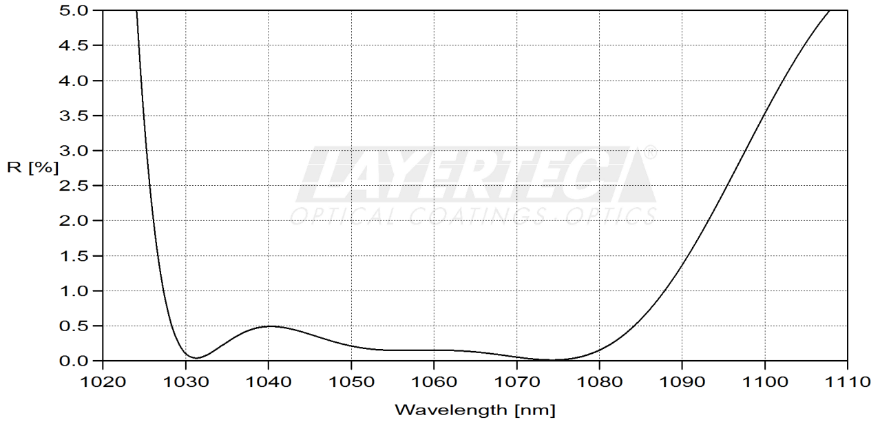
fig. 3 reflection R-region 0°
