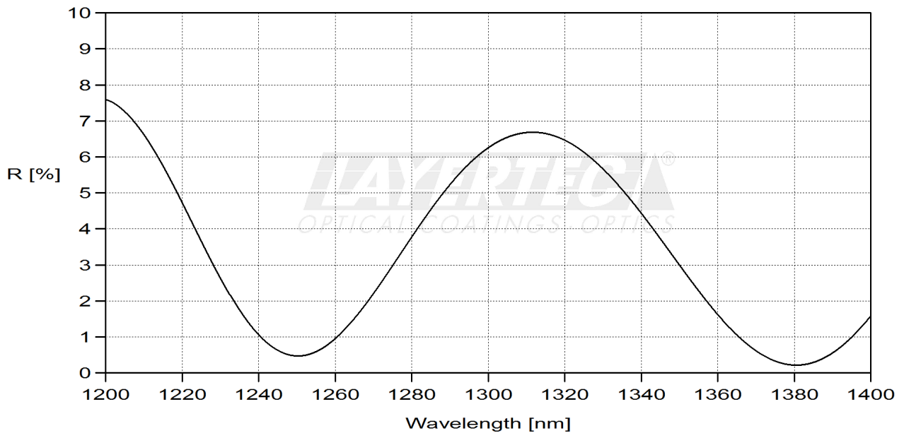
fig. 4 reflection R-region 0°
