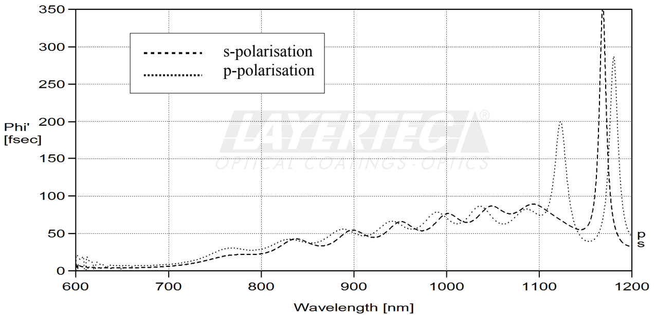
fig. 2 calculated GD(R,45°)
