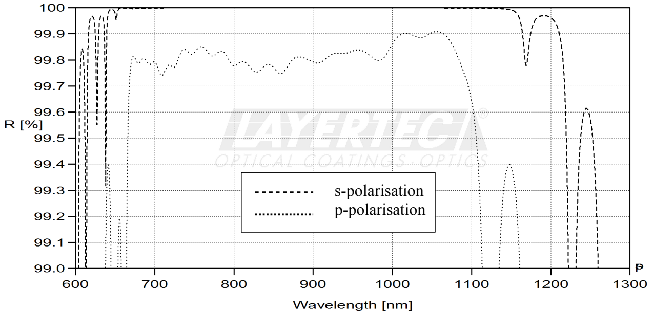
fig. 1 reflection HR-region 45°
