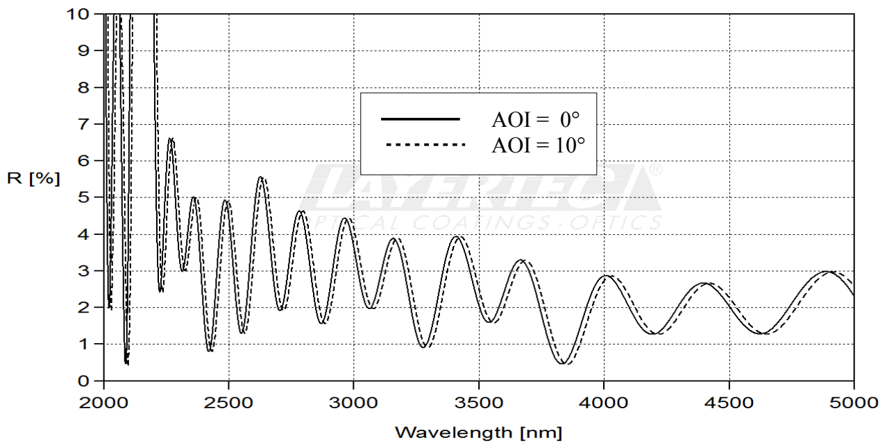
fig. 3 reflection HT-region
