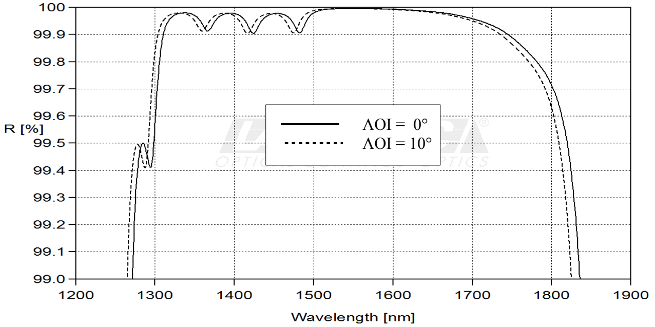
fig. 2 reflection HT-region
