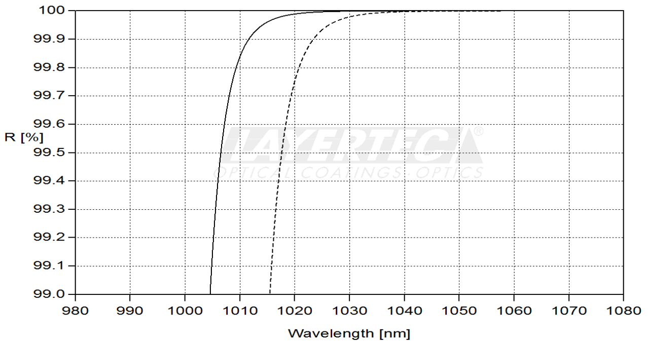
fig. 2 reflection AOI=22.5° detail at HR-region, “—” s-polarized, “-----” p-polarized
