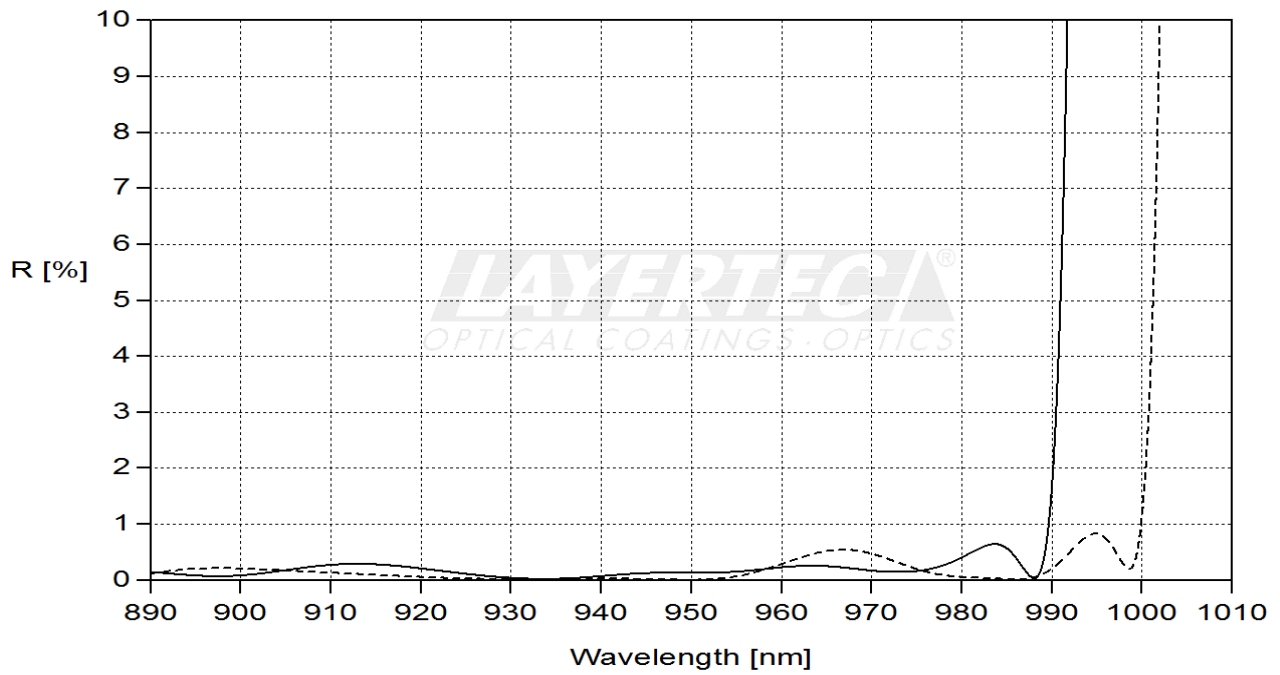
fig. 2 reflection AOI=22.5° detail at R-region, “___” s-polarized, “-----” p-polarized
