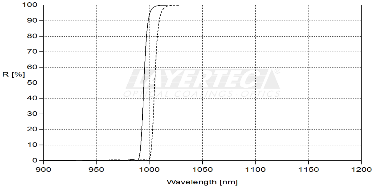
fig. 1 reflection AOI=22.5°, “—” s-polarized, “-----” p-polarized
