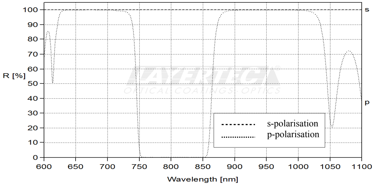
fig. 1 reflection for p- and s-polarisation for AOI=65°
