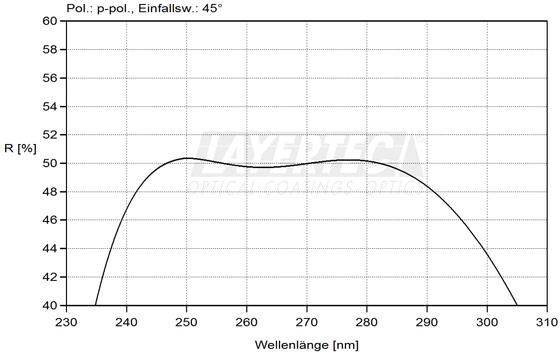
fig. 1: theoretical reflection, p-pol, AOI=45°
