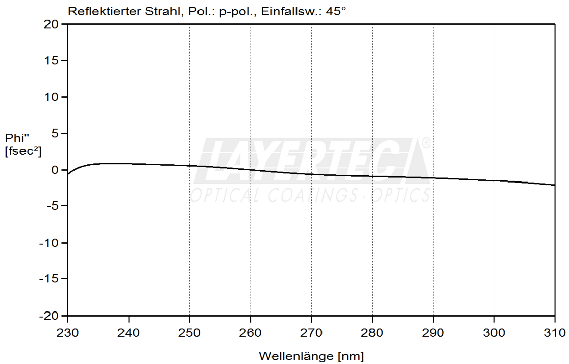
fig. 2: calculated GDD in Reflection, p-pol, AOI=45°
