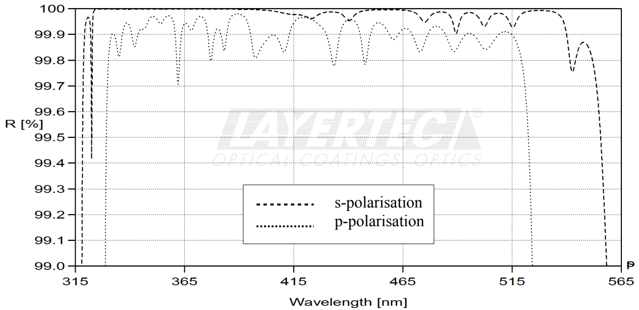
fig. 1 reflection HR-region 45°
