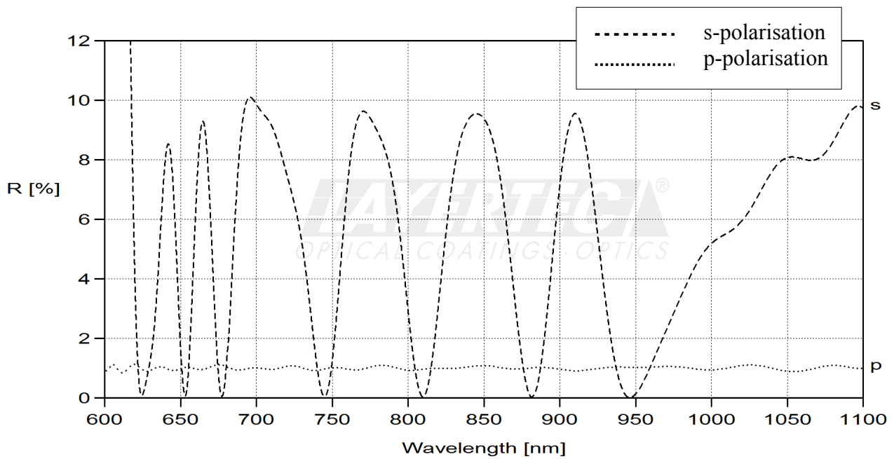
fig. 2 reflection R-region 45°
