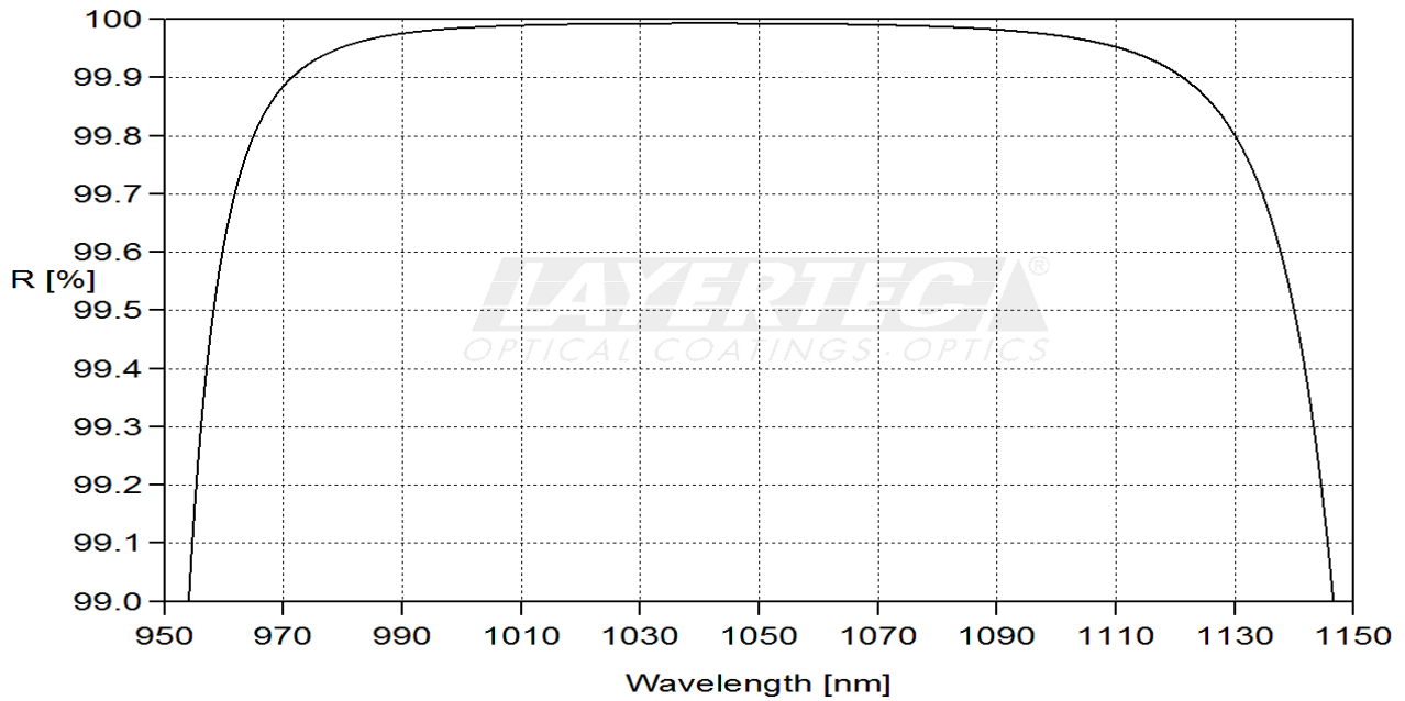
fig. 1 reflection HR-region 22.5° (unpolarized)
