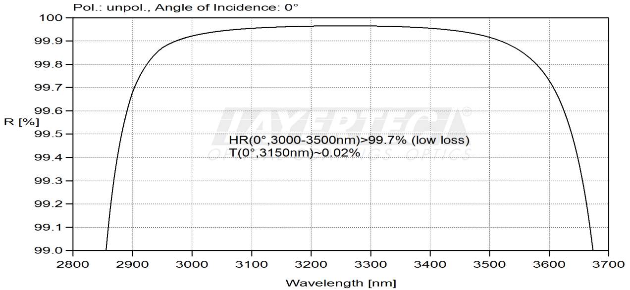
fig. 2 transmission, 0^\circ
