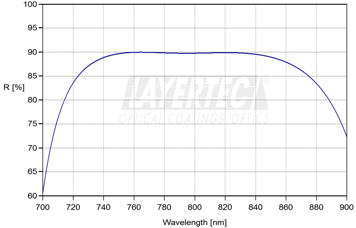
fig. 1.1: PRp (45°, 750-850nm) = 90 ± 3%
