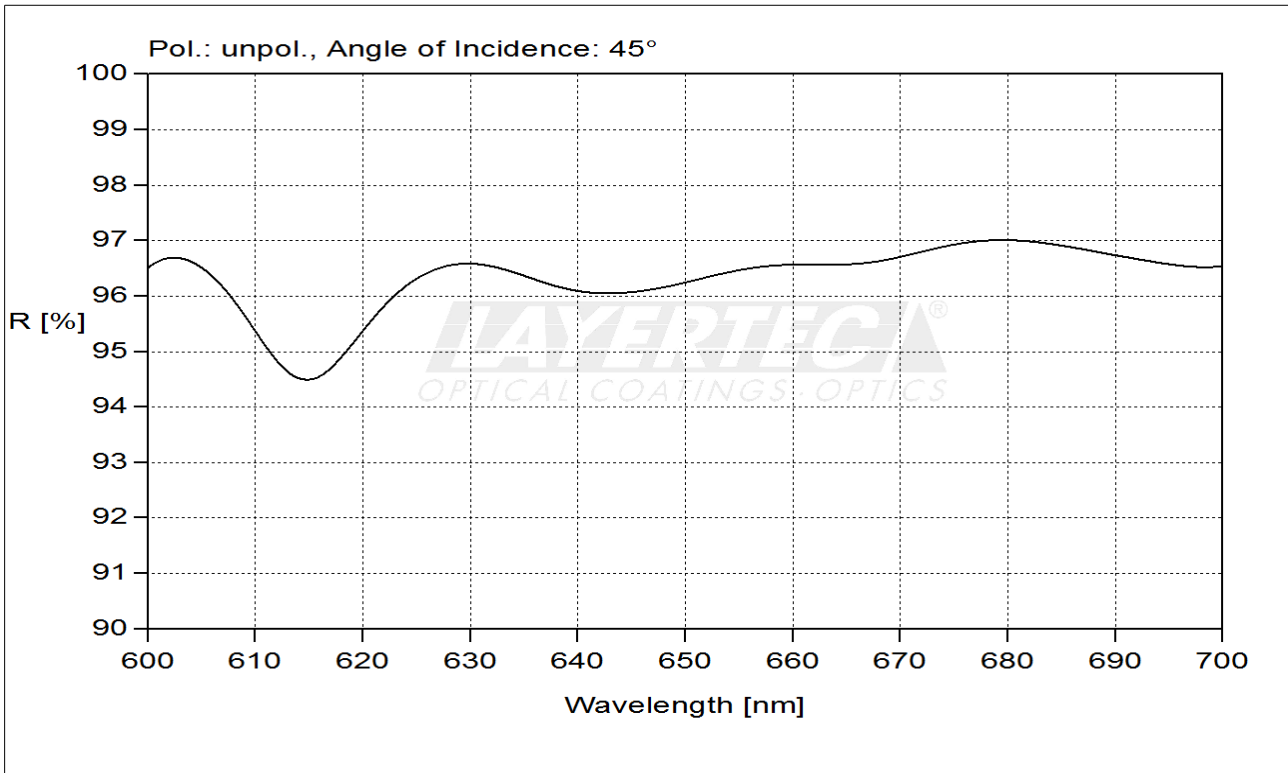
fig. 4: calculated reflectivity @ R region
