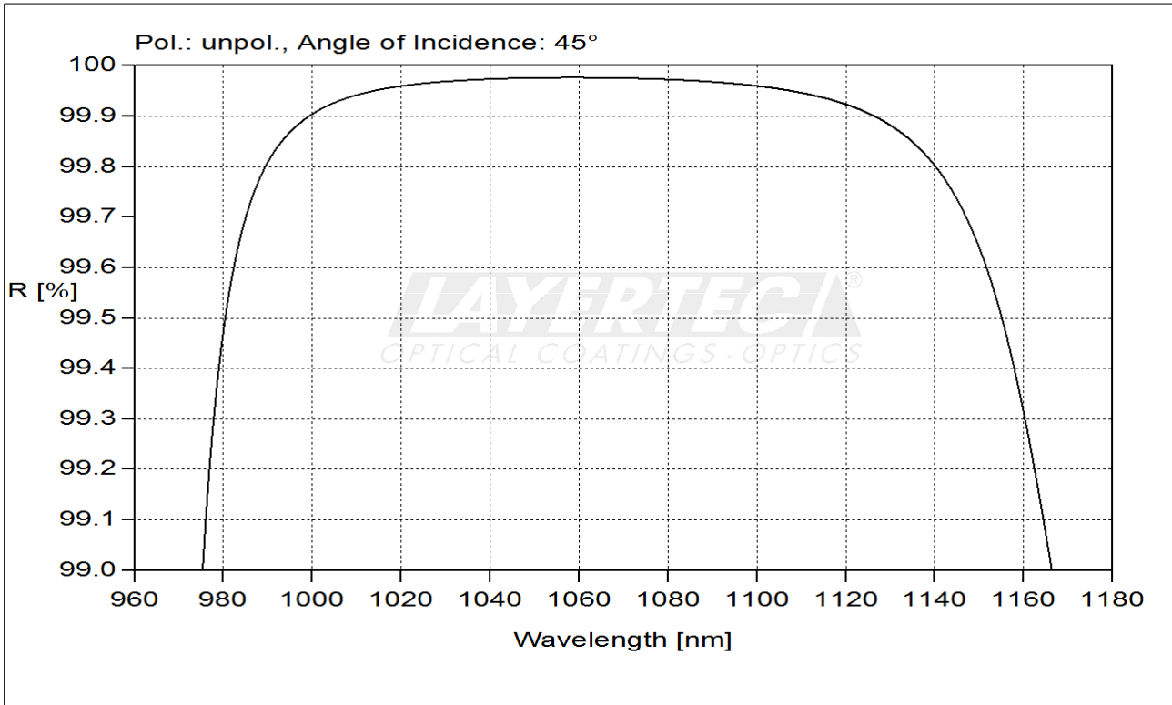
fig. 3: calculated reflectivity @ HR region
