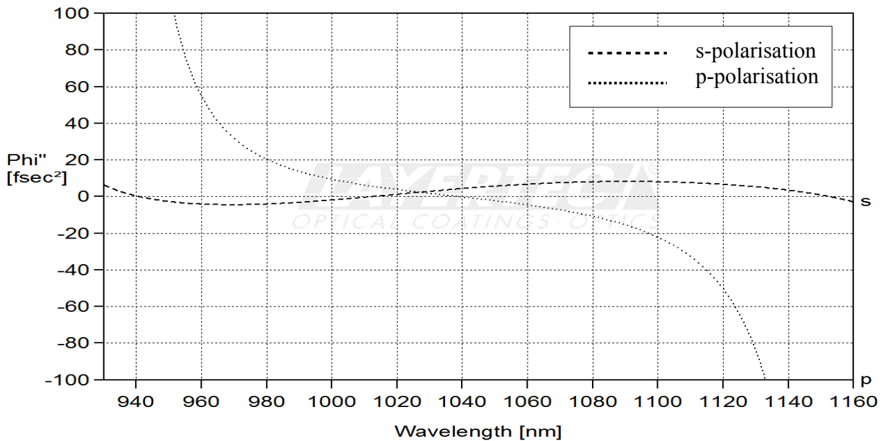
fig. 2 calculated GDD(R,45°)
